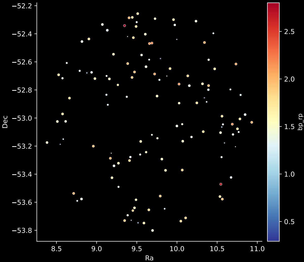
APOGEE DR17 Field: [340-14] Stars: 127
