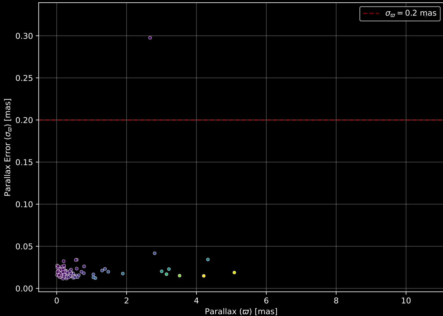
APOGEE DR17 Field: [340-14] Parallax Quality (n= 127)
