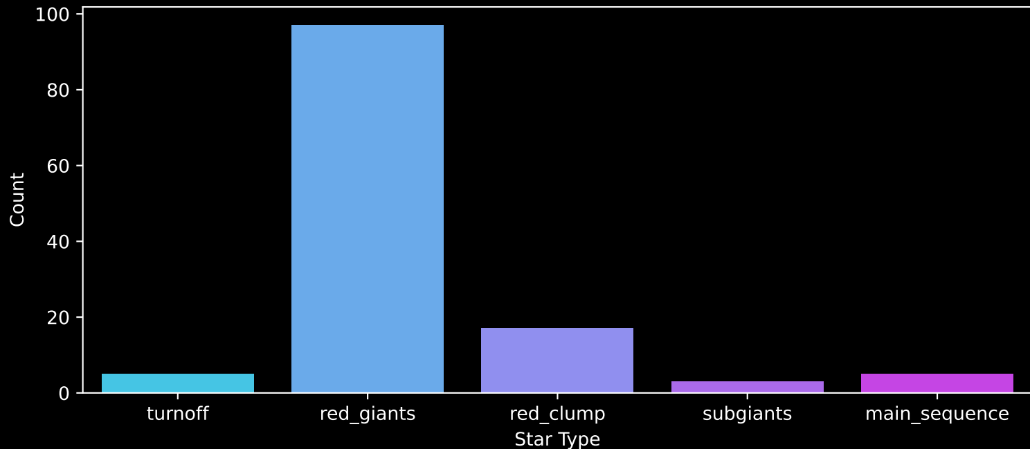
APOGEE DR17 Field: [340-14] Count plot of Star Type
