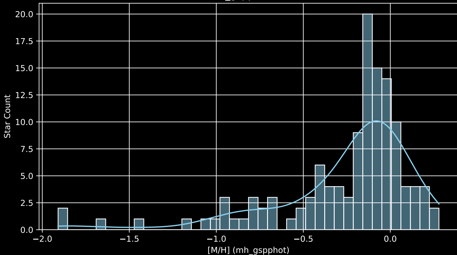
APOGEE DR17 Field: [340-14 [M/H] (mh_gspphot) (n= 125)
