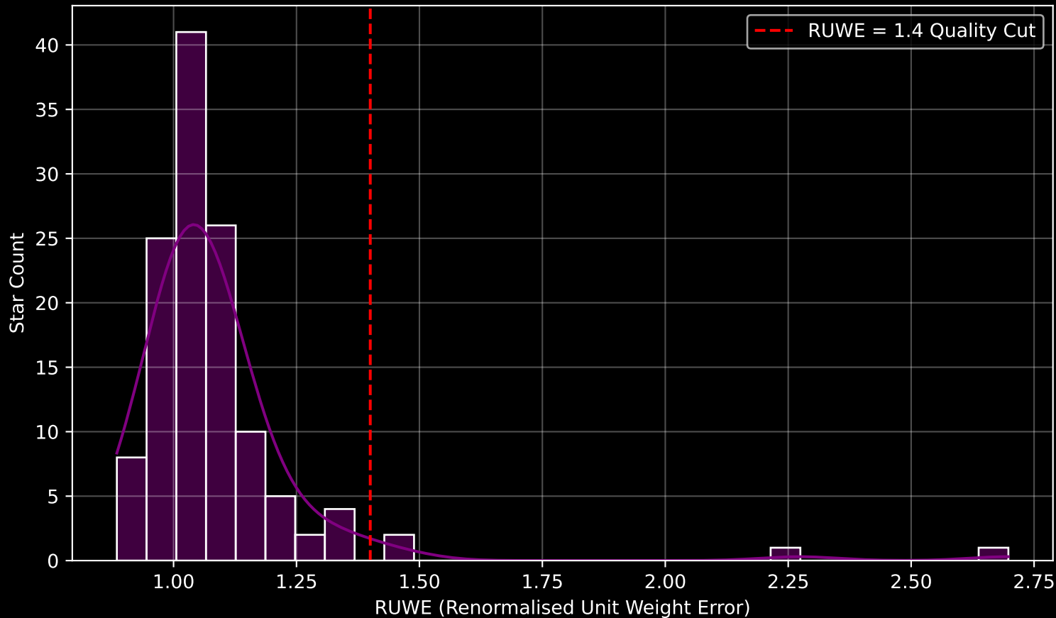
GAPOGEE DR17 Field [340-14] RUWE Distribution (n= 125)
