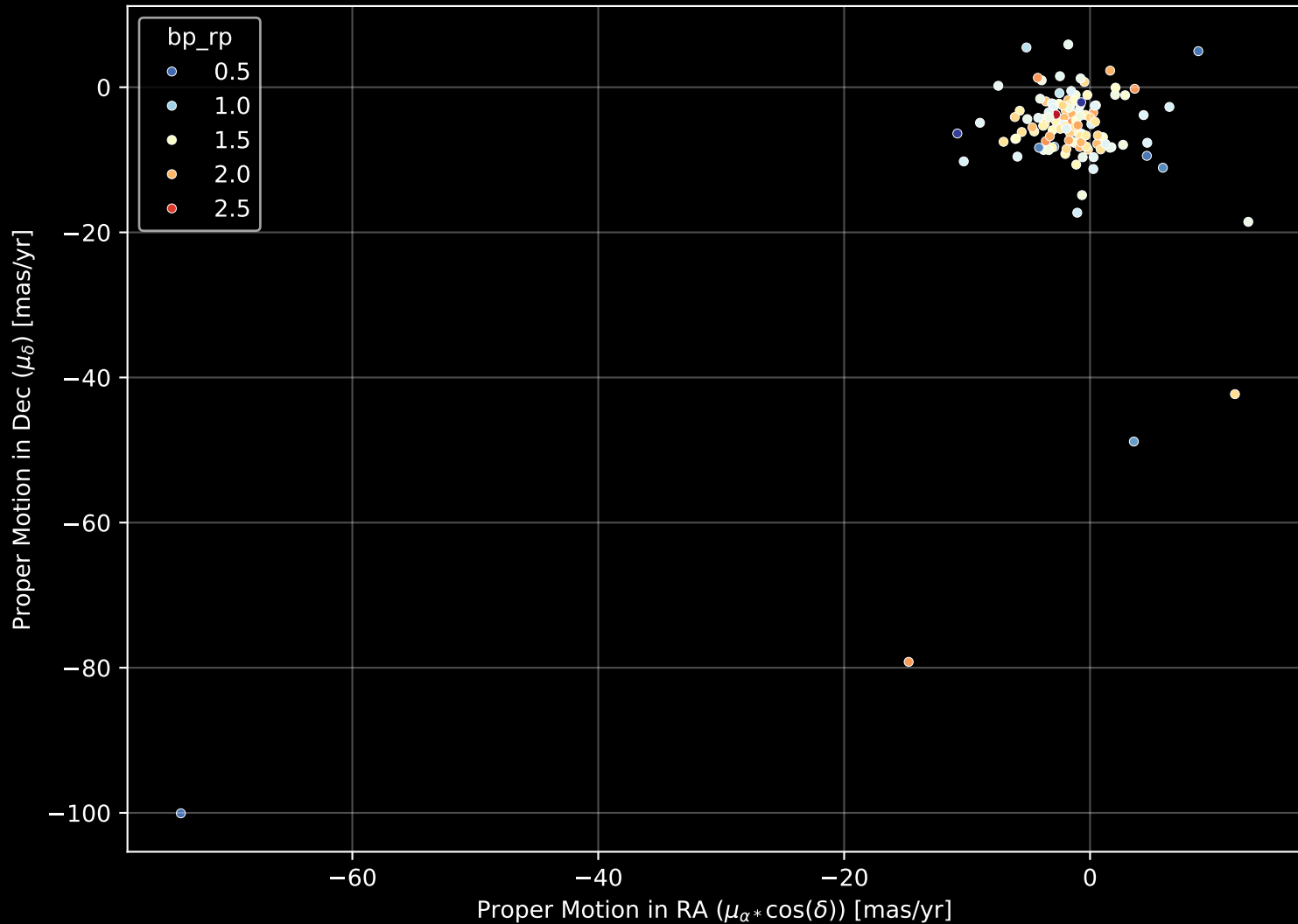
APOGEE DR17 Field: [340-14] Proper Motion Diagram (n= 127)
